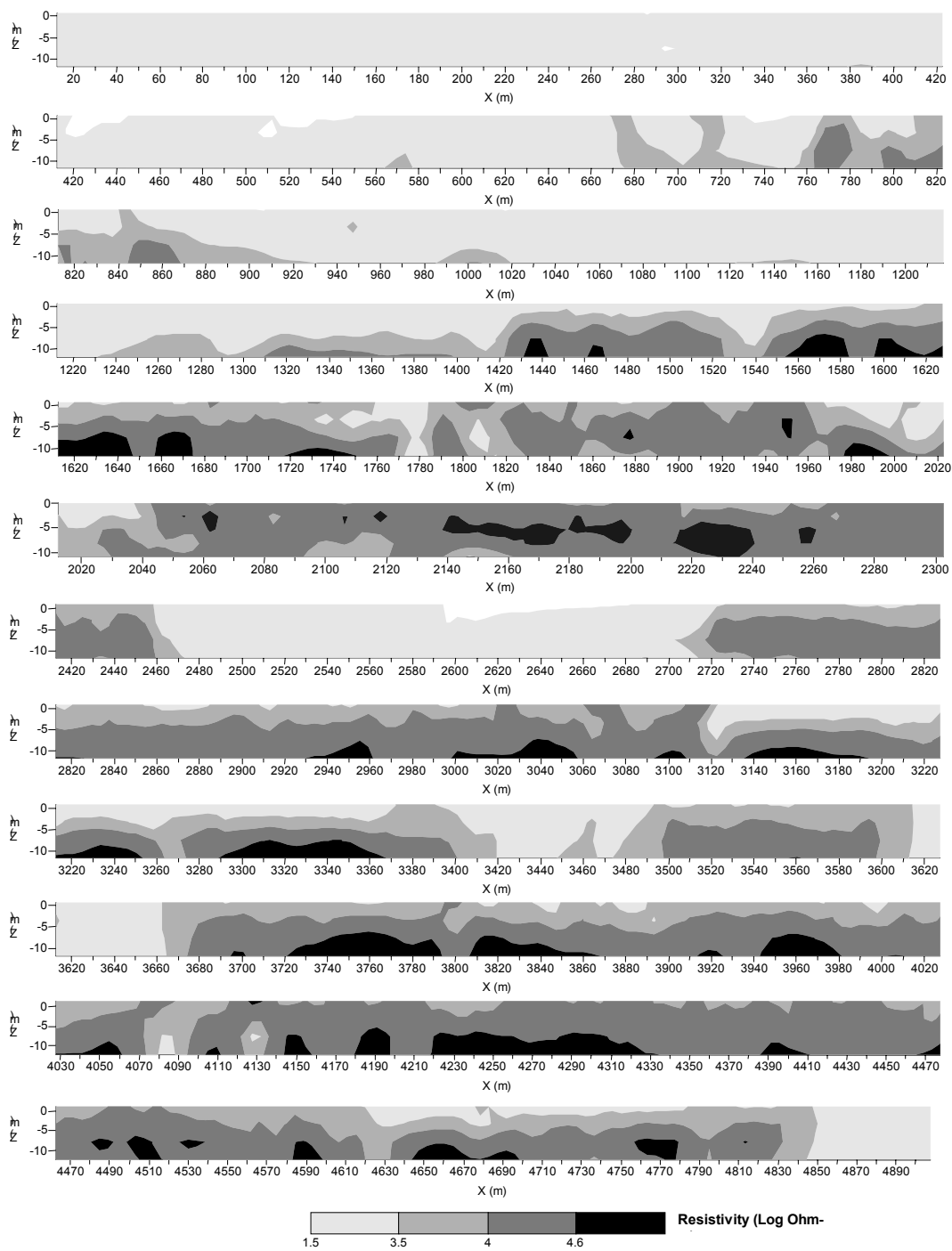
Figure 5: The interpreted geoelectrical image of the entire survey area.
